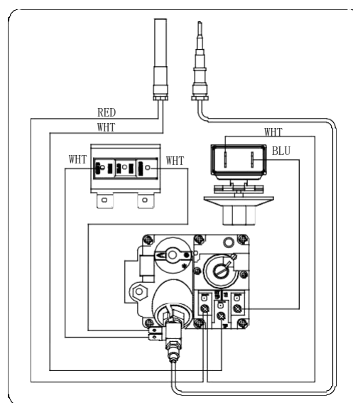
Connection Diagram
