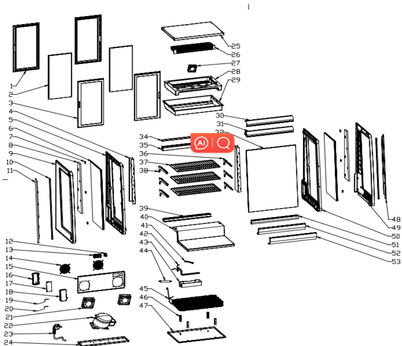
FIGURE 1 FULL OF THE MACHINE
