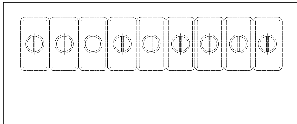
SLB180 1800X750X1080MM
