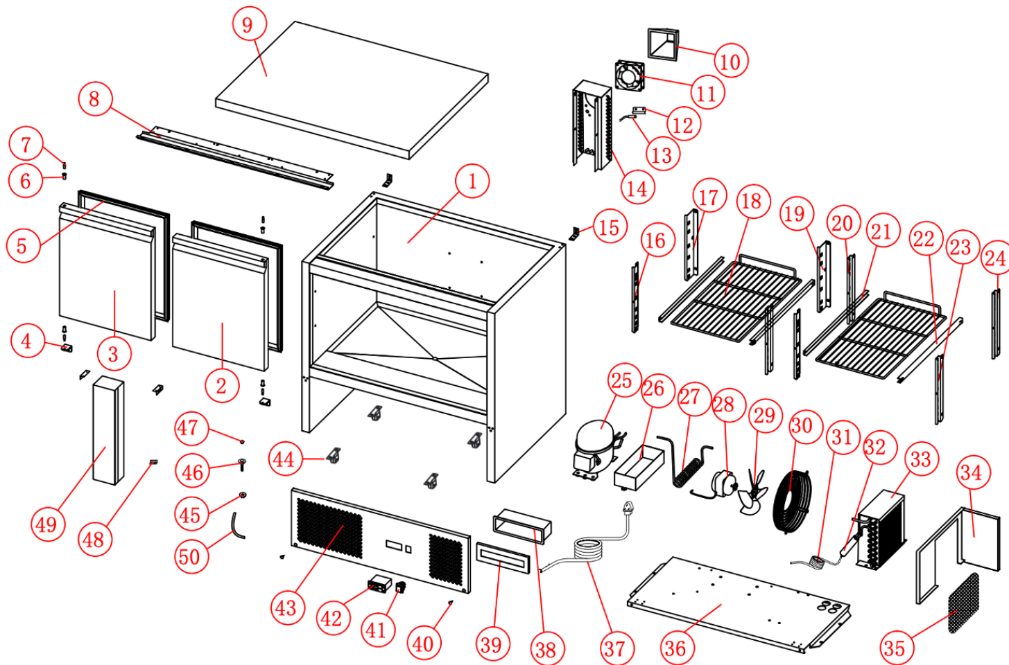
EXPLODED DIAGRAM XGNS900B
