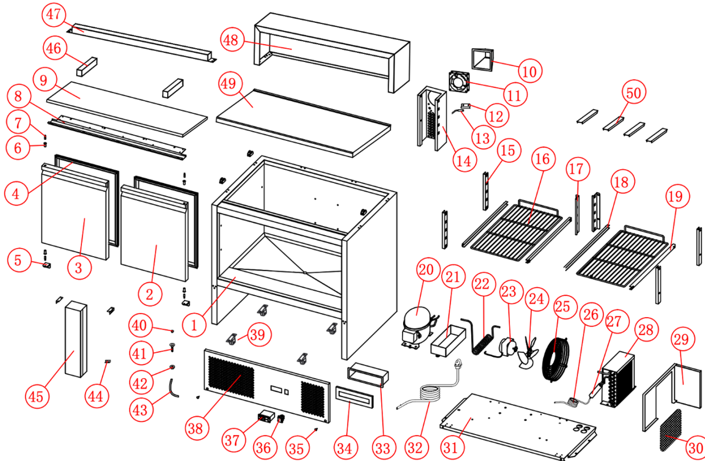
EXPLODED DIAGRAM XGNS900E
