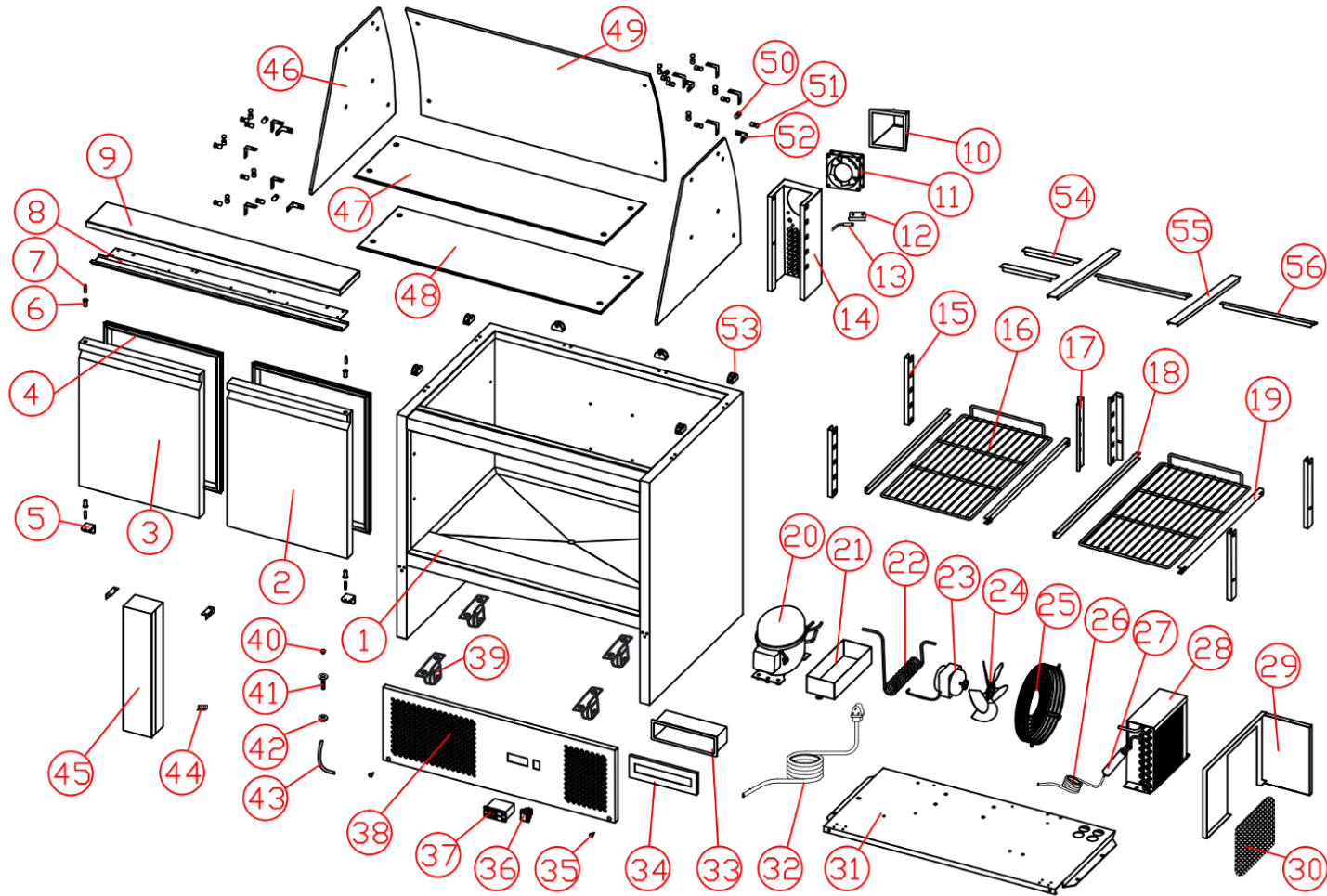
XS900GC EXPLODED DIAGRAM
