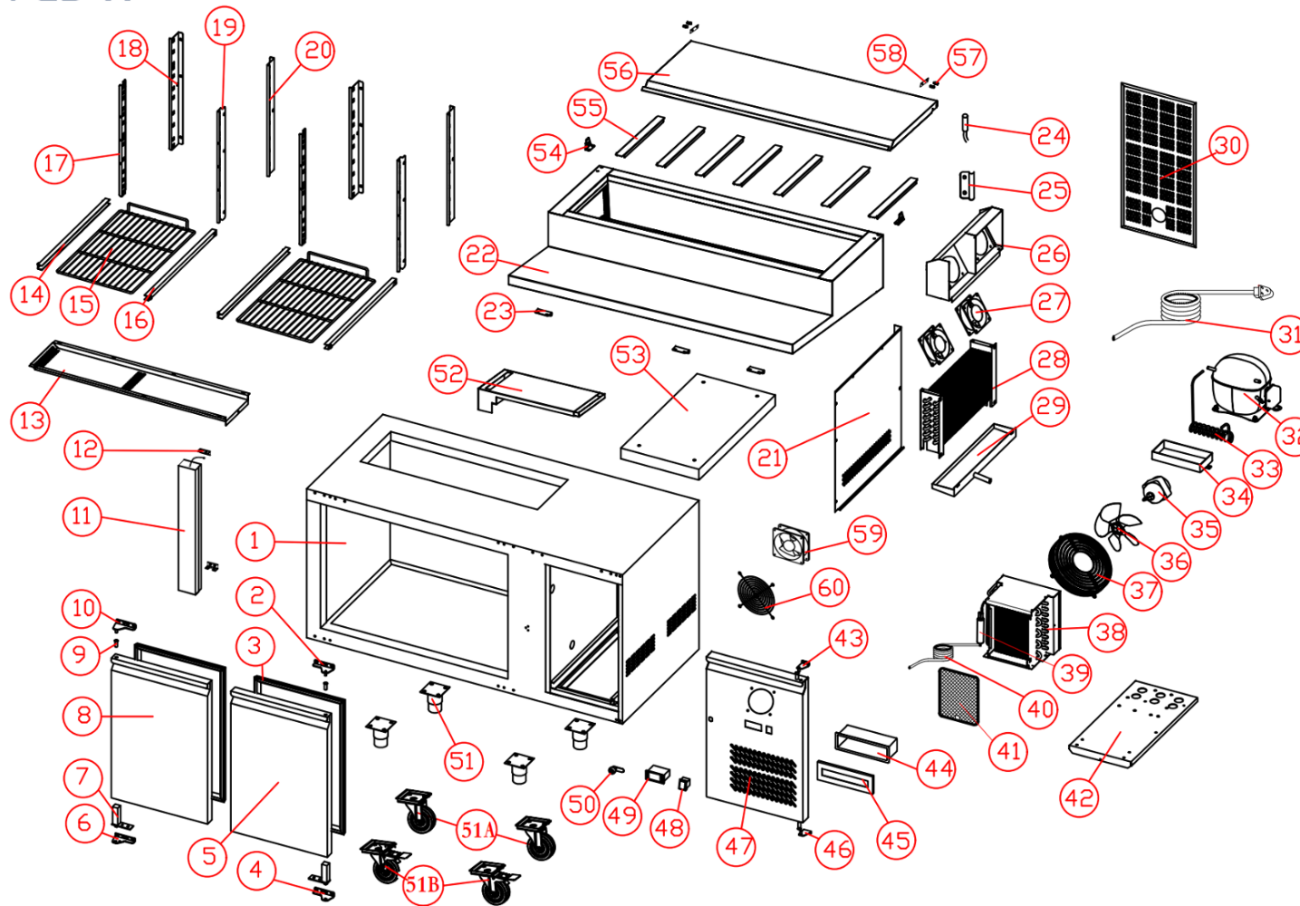
XSS8C15S2V EXPLODED DIAGRAM
