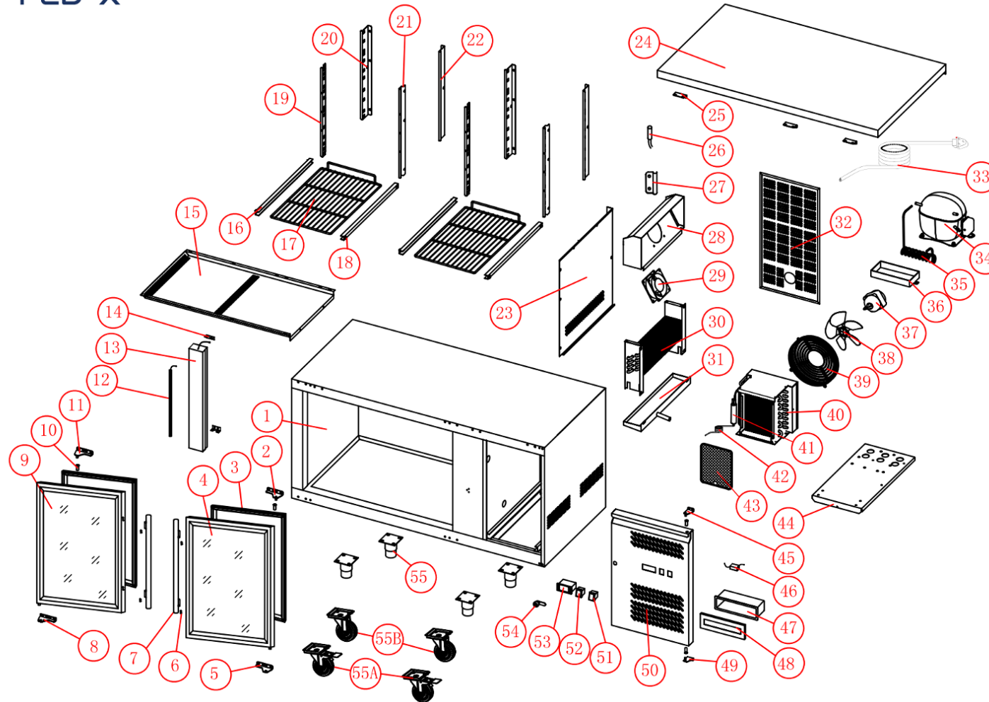
XUB7C13G2V EXPLODED DIAGRAM
