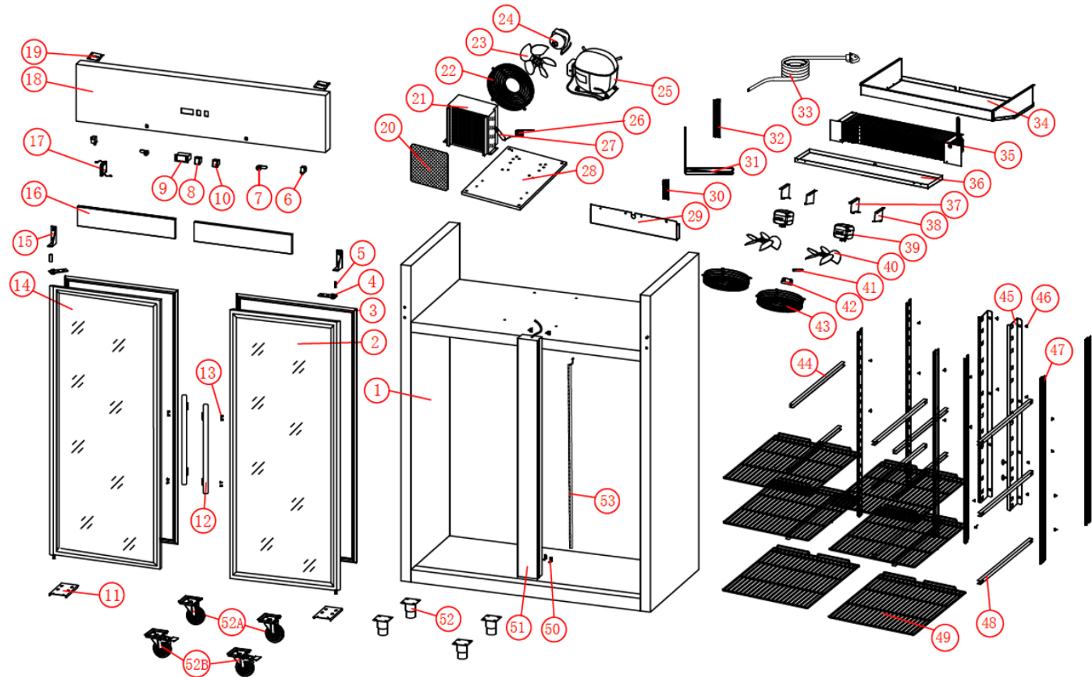
EXPLODED DAIGRAM XURC1200G2V
