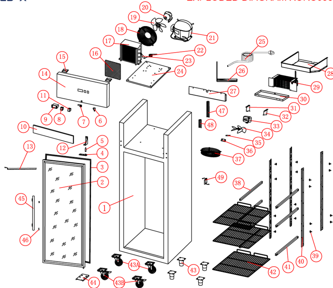
EXPLODED DIAGRAM XURC600G1V
